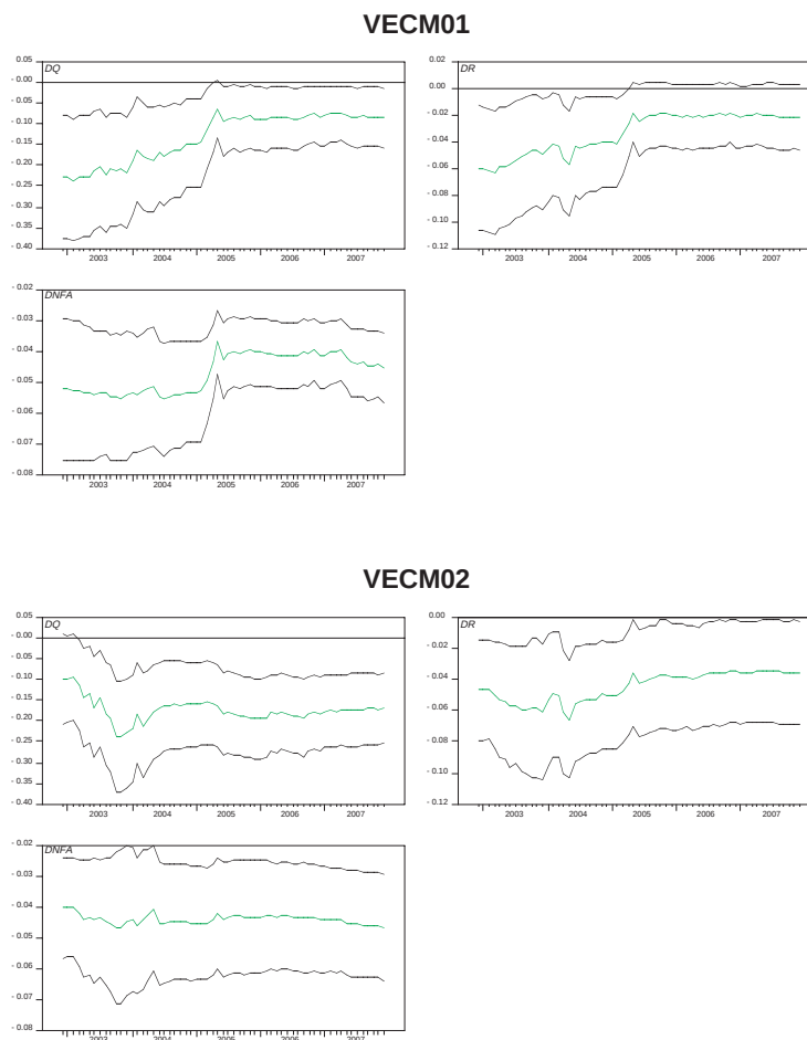
Chart 2: Recursive test for stability of adjustment coefficients
