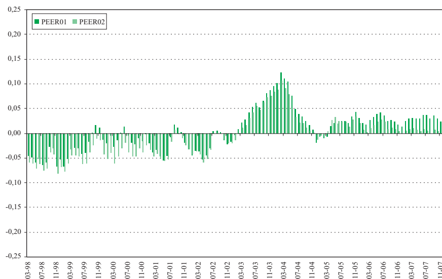
Chart 6: Total misalignment
