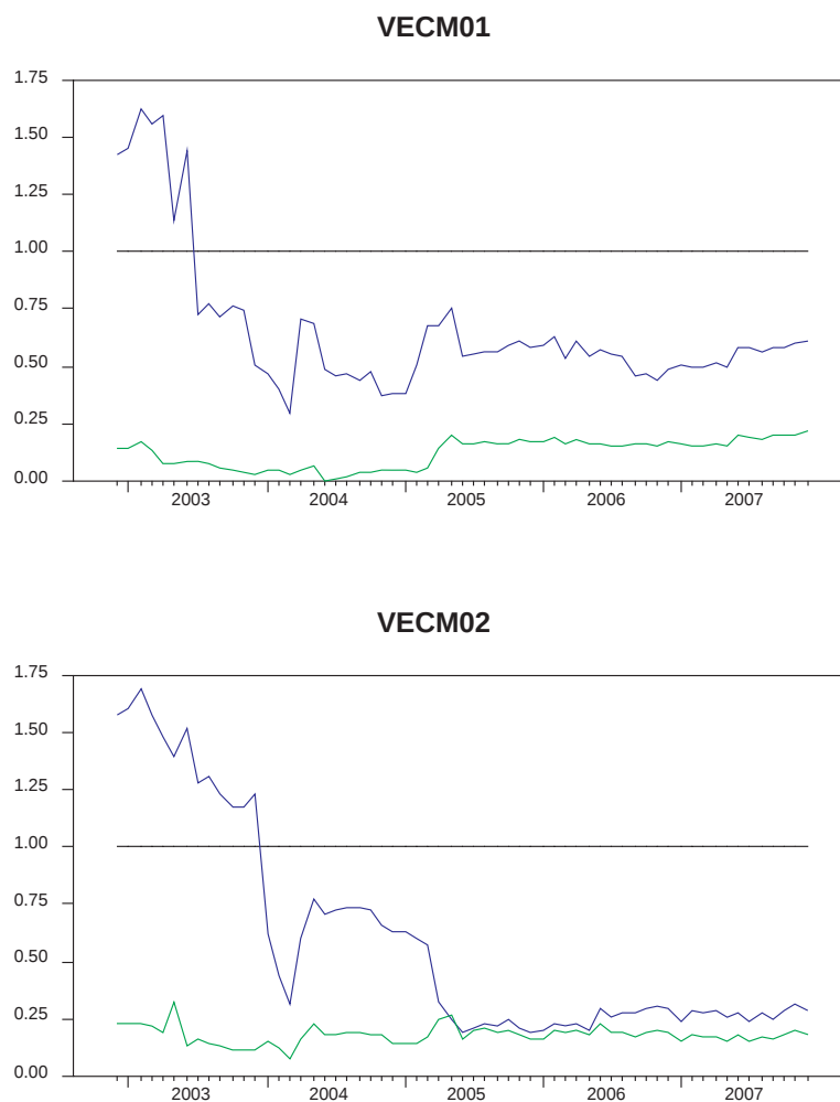
Chart 8: Recursive LR-test of restrictions
